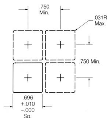
FIGURE 4 MOUNTING PLATE CUTOUT DIMENSIONS TYPE I AND TYPE III SWITCHES
