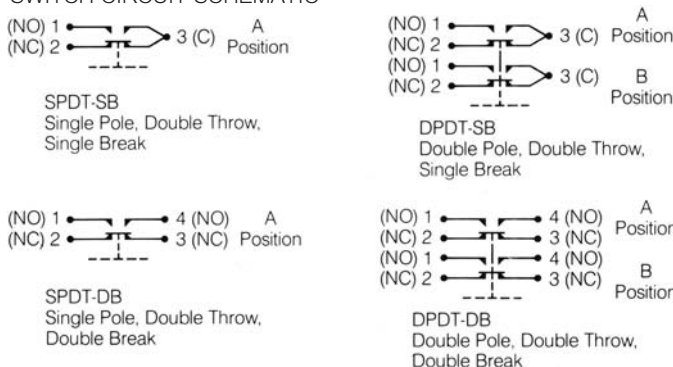
FIGURE 5 SWITCH CIRCUIT SCHEMATIC
