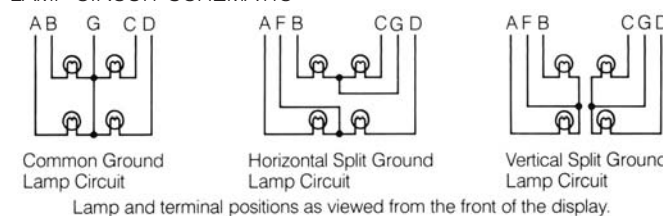
FIGURE 6 LAMP CIRCUIT SCHEMATIC
