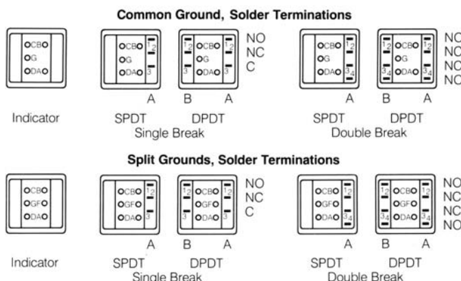
FIGURE 7 SWITCH POLES & LAMP TERMINAL ARRANGEMENTS AND IDENTIFICATION
