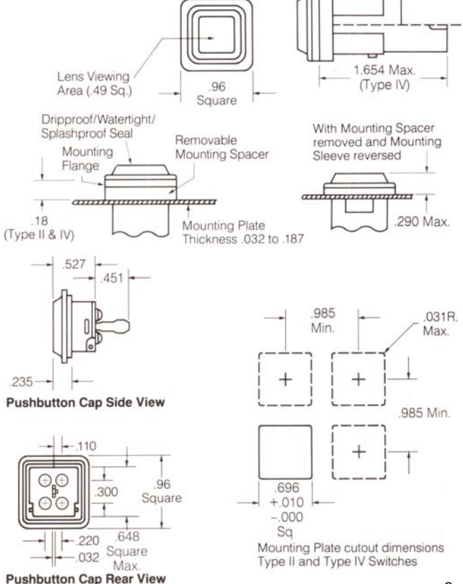
FIGURE 13 SEALED SWITCH DIMENSIONS
